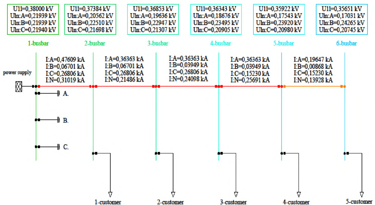
Figure 5. Synchronous compensator connected to Bus 1.
