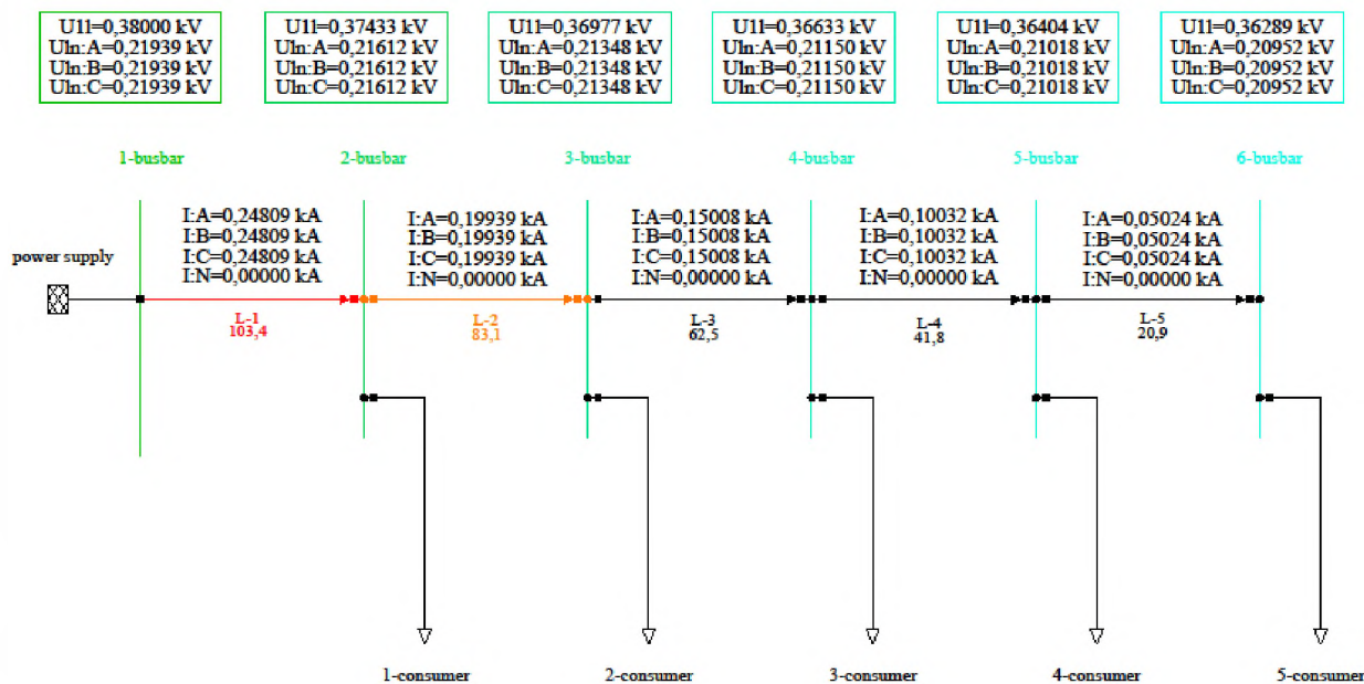
Figure 1. Symmetrical diagram of a 0.38 kV network.
