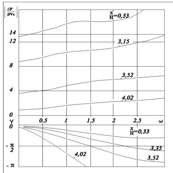
2-rasm. Nostatsionar harakatda bosim moduli va fazaning o'zgarish burchagi \gamma ning Struxal soni \omega ga bog'liqligi.
